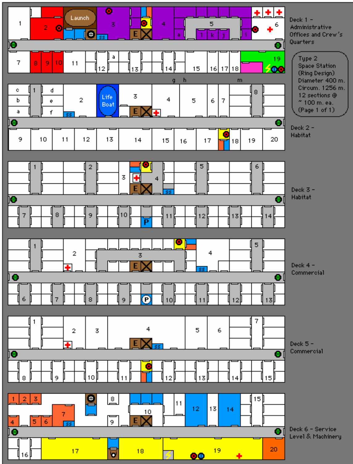
Type 3 Station 600 meter diameter - docks ships hull size 1 thru 14
